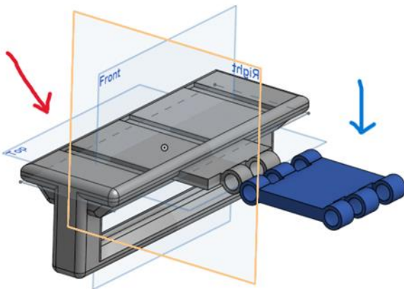
Figure 4. MDCJ magnet holders (indicated by red arrow) and hinges Indicated by blue arrows:
